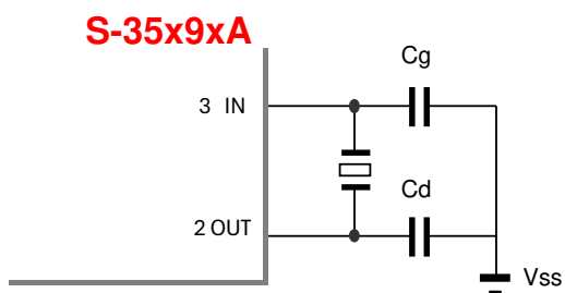
•Circuit Diagram
